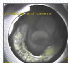
SAND DEPOSIT ON SLIDING SLEEVE
