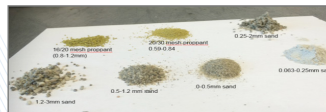
SIMULATED PRODUCED & FRACTURED DEBRIS
